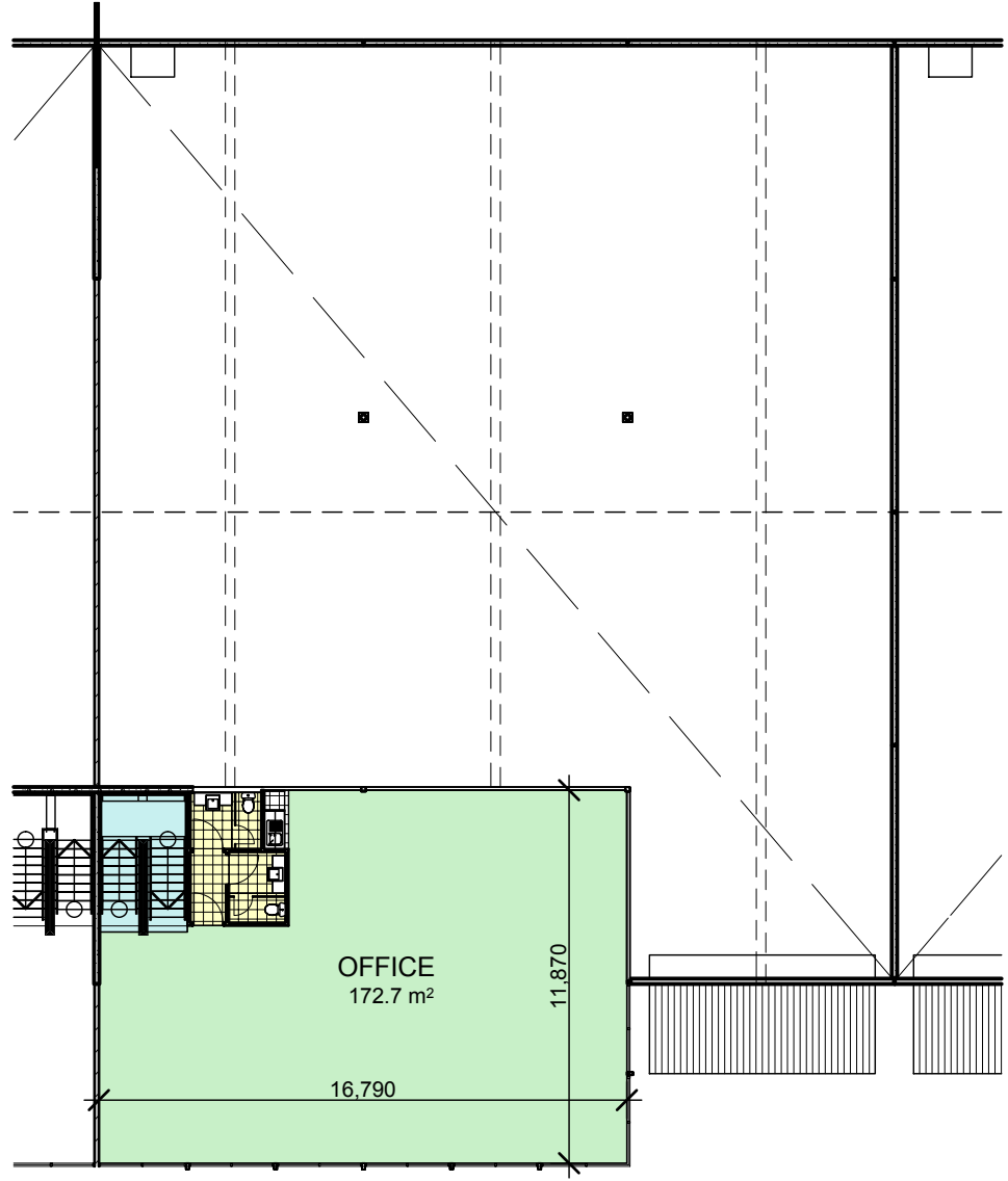
FIRST FLOOR
