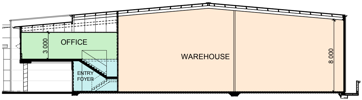
SECTION A
